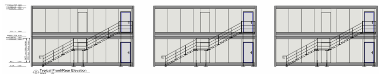
Figure 9-4. Typical Front /Rear Elevation
